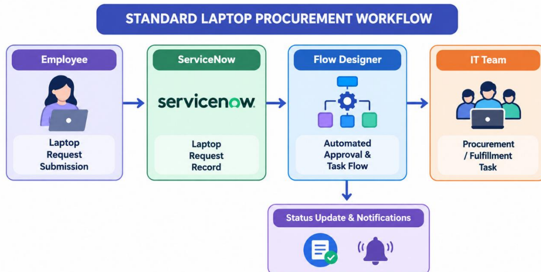
Figure 1: Architecture and workflow of the Standard Laptop Procurement Automation process
